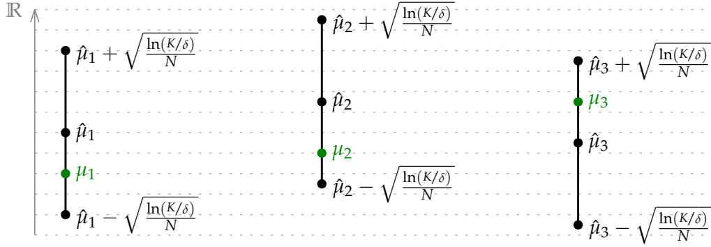
Figure 2.2: Hoeffding inequalities for multiple arms.
