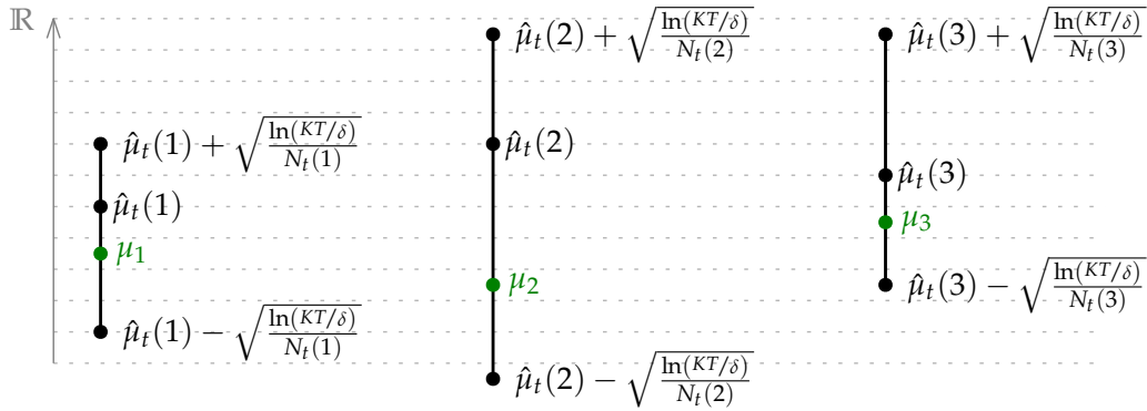
Figure 2.3: In the confidence interval in Equation (2.19), the length depends on how many times one arm has been tried.
