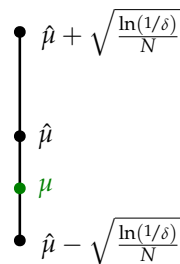
Figure 2.1: The true mean is located at a bounded distance from the sampled mean with probability 1 - \delta .
