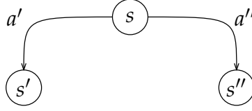
Figure 1.2: Three-states MDP example.
